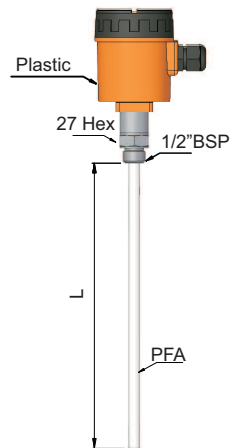
ECAP 101 Fully Insulated Conductive Tank
